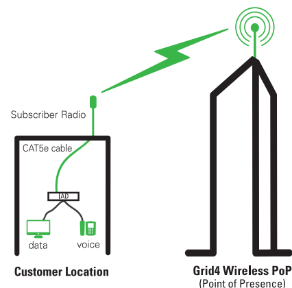
How Fixed Wireless Broadband Works
